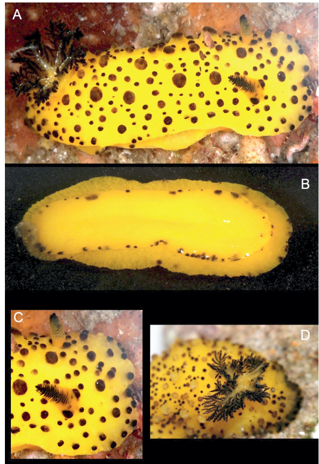
Figure 1 Doris ananas live specimen. A. Dorsal-slightly right view. B. Ventral view. C. Detail anterior region, dorsal-slightly right view. D. Detail of extended gill circle, dorsal view.
